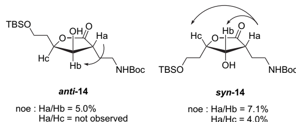
Figure 4. Determination of relative stereochemistry of 14 by NOE-difference experiment.
