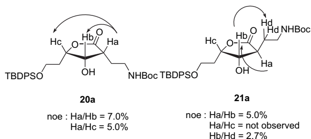
Figure 5. Determination of relative stereochemistry of 20a and 21a by NOE-difference experiment.
