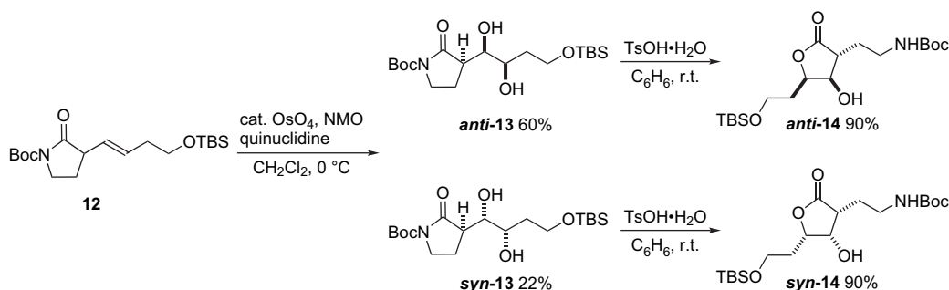
Scheme 7. Synthesis of 2,4-dialkyl-3-hydroxybutanolide 14 .
