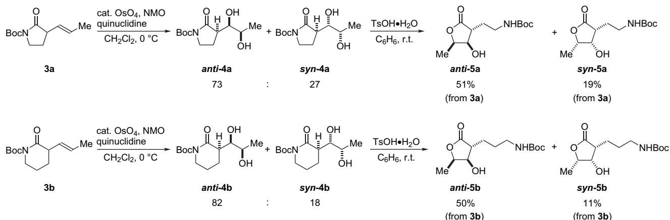
Scheme 4. Acid-catalyzed ring-switch reaction of 3a and 3b .
