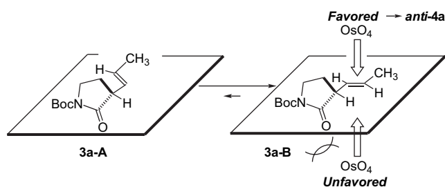
Figure 2. Stereoselective osmylation of 3a .
