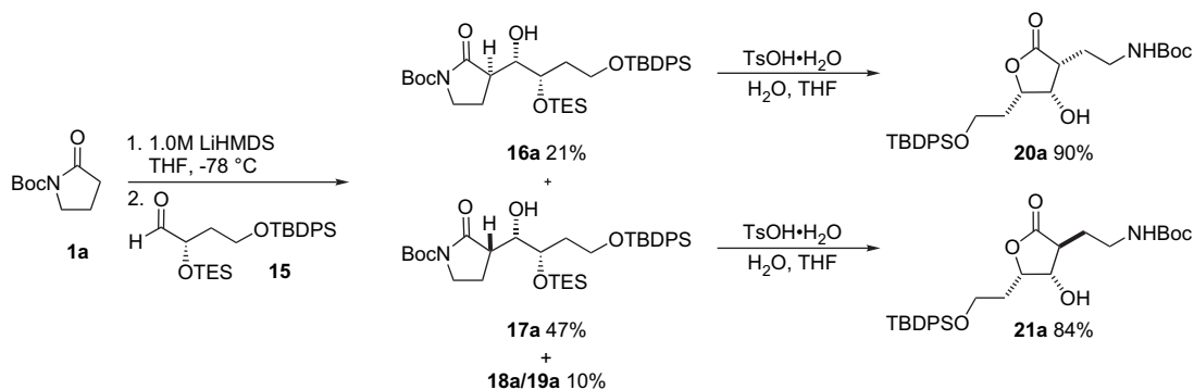
Scheme 8. Syntheses of chiral 2,4-dialkyl-3-hydroxybutanolides.
