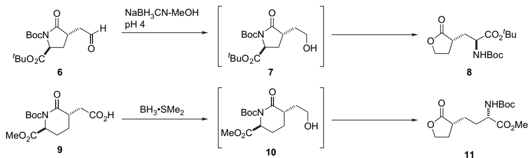
Scheme 5. Reported ring-switch reaction by Young and co-workers. 10
