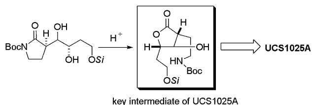
Scheme 6. Synthetic approach to the key intermediate of UCS1025A.
