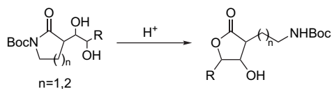
Scheme 1. Acid-catalyzed ring-switch reaction of 2-(2-hydroxyalkyl)lactams to 2,4-dialkyl-3-hydroxybutanolides.
