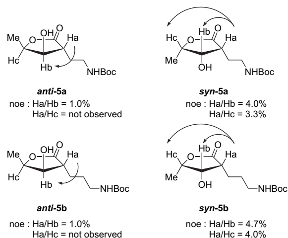
Figure 3. Determination of relative stereochemistry of 5 by NOE-difference experiment.
