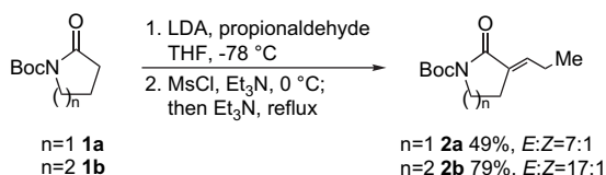
Scheme 2. Syntheses of 2-propylenelactams by aldol condensation.
