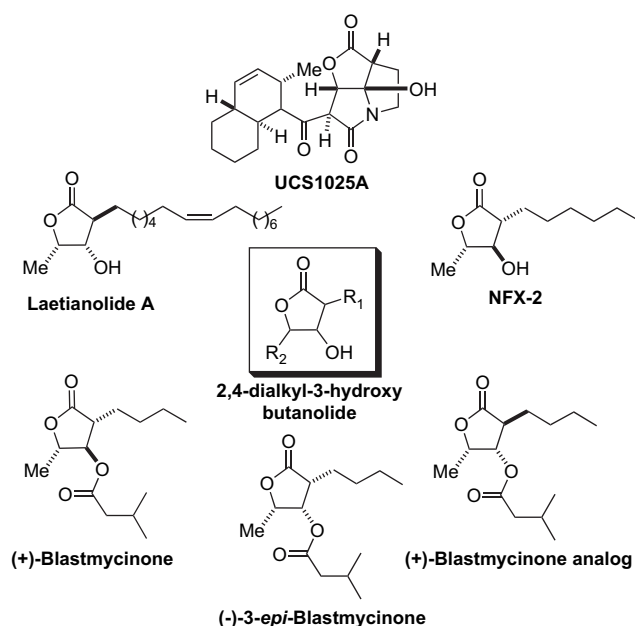
Figure 1. 2,4-Dialkyl-3-hydroxybutanolide natural products and derivatives.
